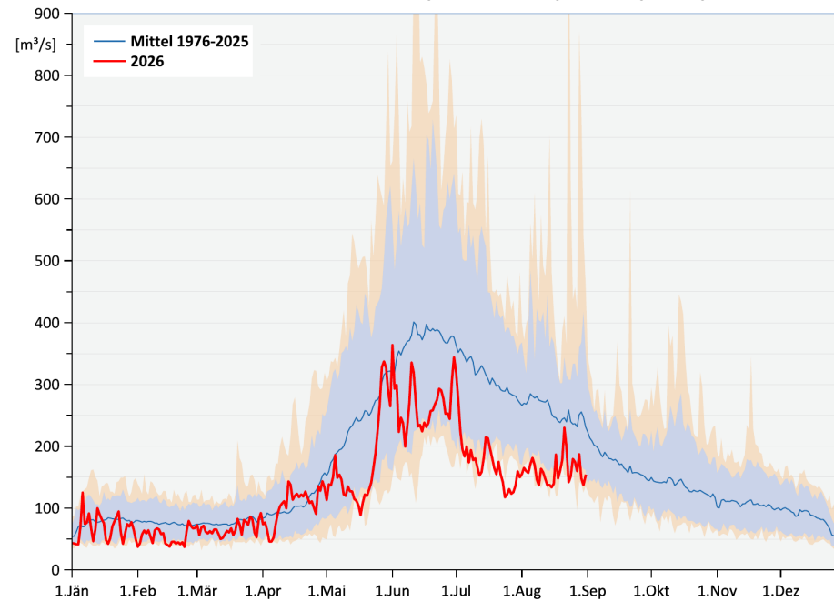
201525 Innsbruck (oberh. Sill) / Inn (Tirol)
